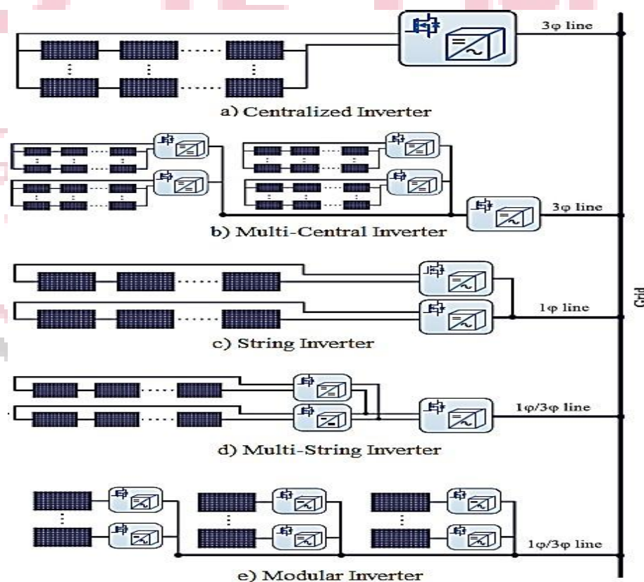
Figure 1.1 Grid Connected PV Topologies
