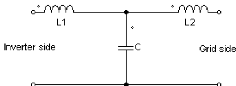
Figure 5.1: An LCL filter
