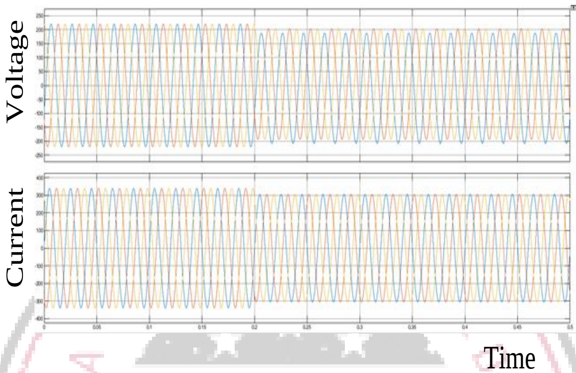
Figure 6.2: Three phase AC load voltage and current
